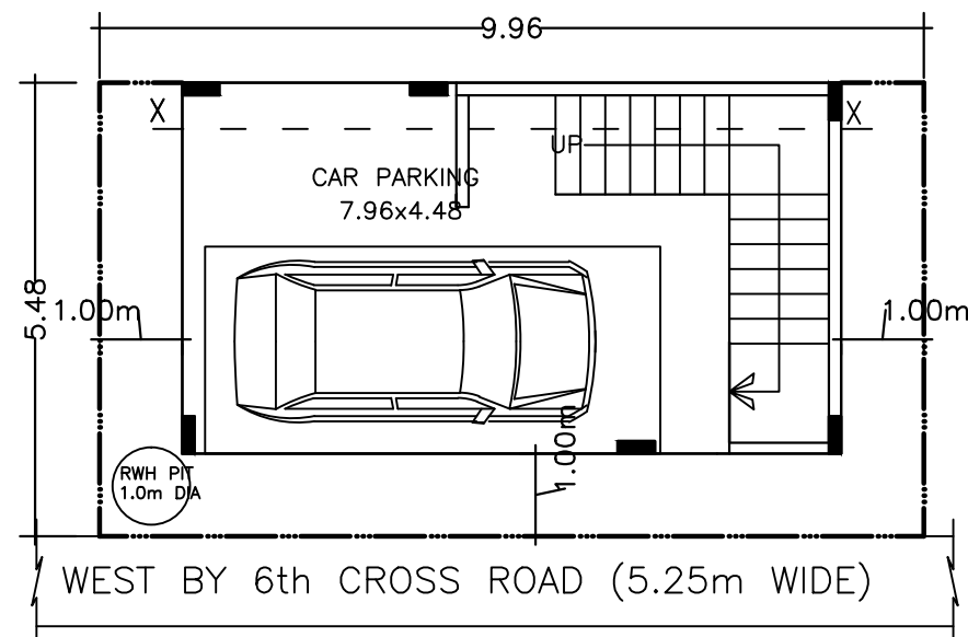
STILT FLOOR PLAN
