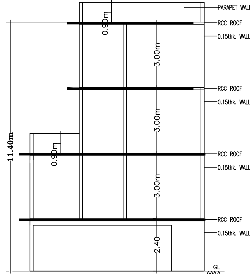
SECTION@X-X
